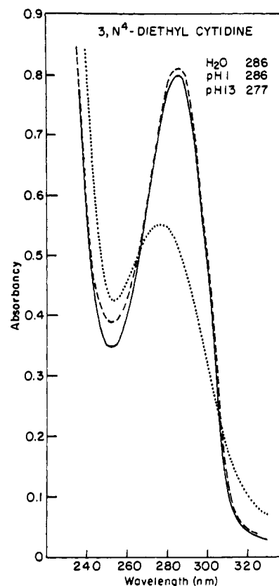
FIGURE 3: Ultraviolet absorption spectra of 3, N^4 -diethylcytidine in water (—), 0.1 N HCl (---), and 0.1 N KOH (.....). The absorption maximum at each pH is given in the figure.
