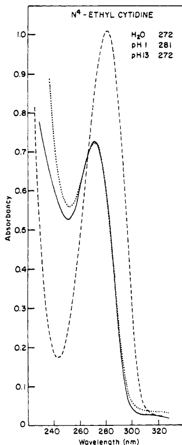
FIGURE 2: Ultraviolet absorption spectra of N^4 -ethylcytidine in water (—), 0.1 N HCl (---), and 0.1 N KOH (.....). The absorption maximum at each pH is given in the figure.
