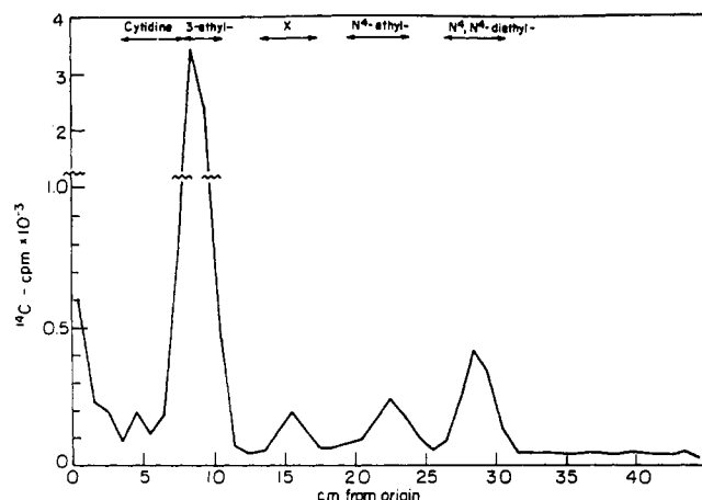
FIGURE 8: Radioactivity profile of a chromatogram of poly(C) reacted with [^{14}\text{C}]\text{EtMeSO}_3 . See text for experimental details. One-third of the sample, after repeated alcohol precipitation, was enzyme digested to nucleosides and chromatographed in solvent B. Double arrows indicate the positions of ultraviolet-absorbing internal markers. Radioactivity was determined as in Figure 6.
