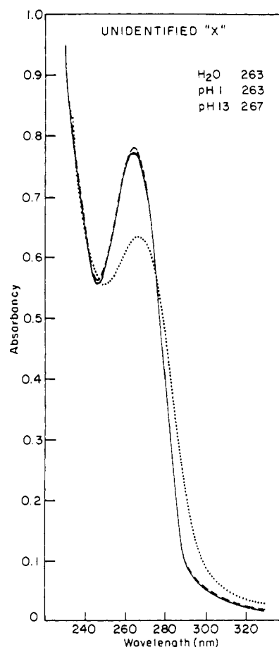
FIGURE 7: Ultraviolet absorption spectra of unidentified ethylcytidine "X" in water (—), 0.1 N HCl (---), and 0.1 N KOH (.....). The absorption maximum at each pH is given in the figure.
