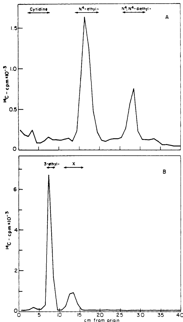
FIGURE 6: Radioactivity profiles of chromatograms of electrophoretic fractions of cytidine reacted with ^{14}\text{C} -EtMeSO 3 . Cytidine (50 mg) was reacted at pH 7.0 with a total of 20 \mu\text{l} of ^{14}\text{C} -EtMeSO 3 (specific activity 1 Ci/mol) for 24 hr at room temperature. Paper electrophoresis of 20% of the ether-extracted solution was in 0.05 M ammonium formate buffer at pH 5.7. (A) Twenty-five per cent of the electrophoretic "low pK" fraction was chromatographed in solvent B. (B) Three per cent of the electrophoretic "high pK" fraction was chromatographed in solvent B. The chromatograms were cut into 1-cm strips and counted in toluene containing Omnifluor (14.7 g/3 l. of toluene) in a Beckman liquid scintillation counter. Double arrows indicate the positions of ultraviolet absorbing internal markers.
