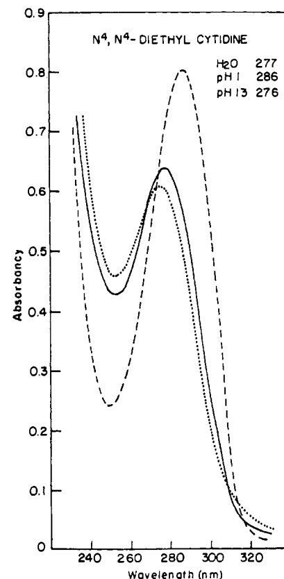
FIGURE 4: Ultraviolet absorption spectra of N^4 , N^4 -diethylcytidine in water (—), 0.1 N HCl (---), and 0.1 N KOH (.....). The absorption maximum at each pH is given in the figure.
