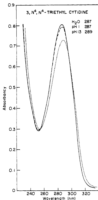
FIGURE 5: Ultraviolet absorption spectra of presumed 3, N^4 , N^4 -triethylcytidine in water (—), 0.1 N HCl (---), and 0.1 N KOH (·····). The absorption maximum at each pH is given in the figure.
