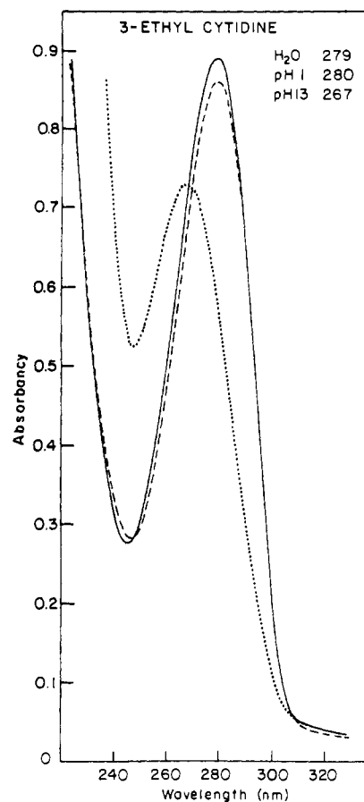
FIGURE 1: Ultraviolet absorption spectra of 3-ethylcytidine in water (—), 0.1 N HCl (---), and 0.1 N KOH (·····). The absorption maximum at each pH is given in the figure.
